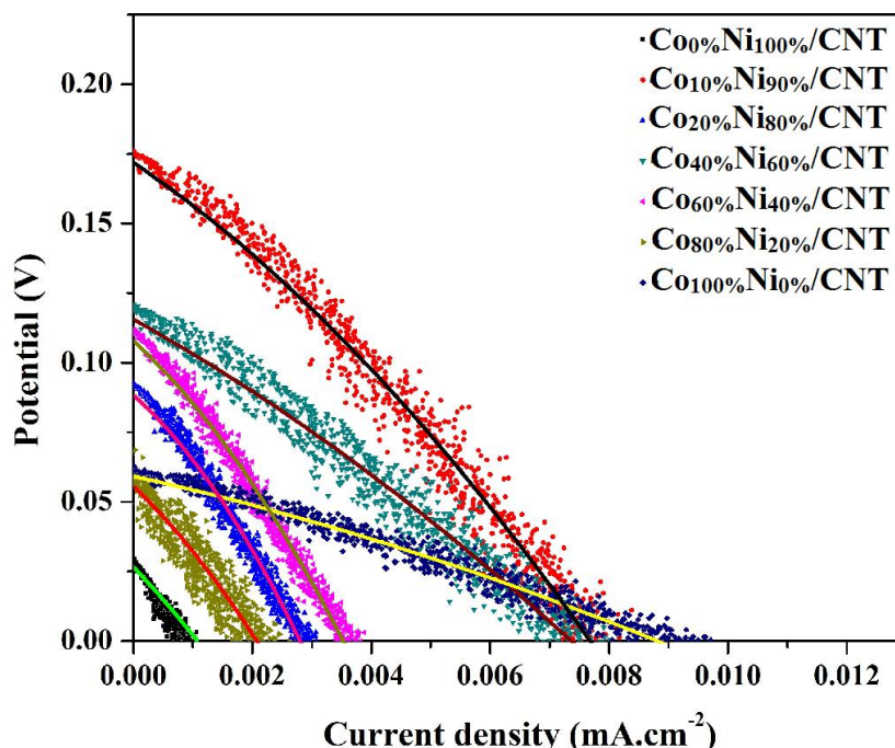
Figure 3. Polarization curve for the direct fuel cell using different composition metal nanoparticle/CNT anodes: Real data and the corresponding polynomial fittings. The polarization curves have been measured at 1 mV/s scan rate at room temperature ( \sim 17^\circ\text{C} ). Normalization of the current was carried out with respect to the anode apparent surface area.
