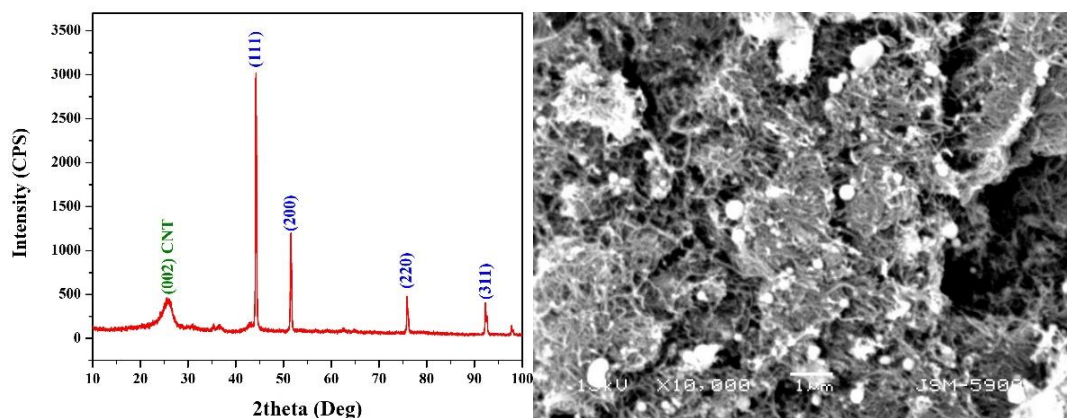
Figure 2. XRD pattern; (A) and SEM image; (B) of the CoNi nanoparticles / CNT composite. The Miller indices of the crystal were added in the XRD pattern
