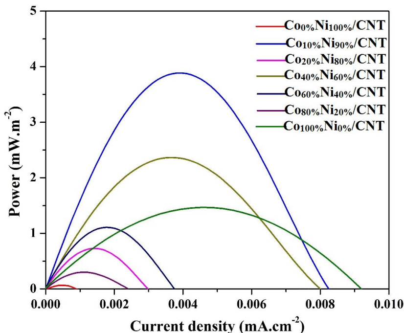
Figure 4. Power density curves for direct fuel cells using different composition metal nanoparticle/CNT anodes. The power density was estimate from the polarization curves which were measured at 1 mV/s scan rate at room temperature (~ 17 °C). Normalization of the power was carried out with respect to the anode apparent surface area.
