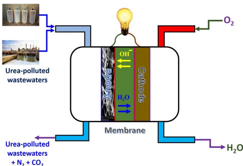
Figure 1. Schematic diagram for the utilization of the direct urea fuel cells.
