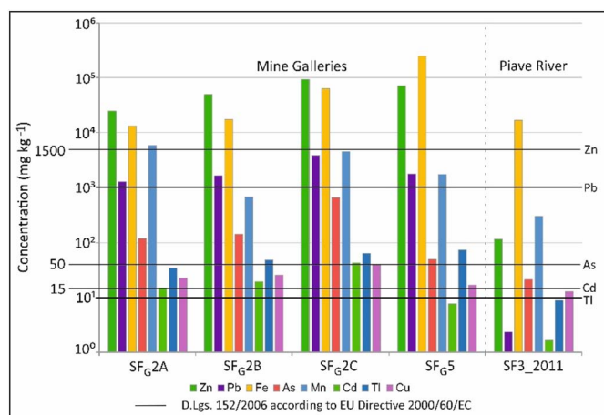
Fig. 6. Comparison of PHEs concentrations observed in fine sediment samples collected at the bottom of the mine galleries and at the banks of the Piave River.
