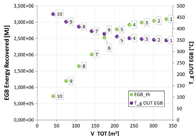
Fig. 10. Annual average energy recovered by EGB use and exhaust gas Temperature (T_g OUT EGB) vs. total volume occupied for every #EGB.
