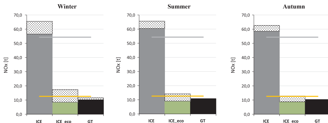
Fig. 11. Overall cruise NO x emissions for every season and engines’ configuration compared with Tier II (bold upper line) and Tier III (bold lower line) emissions, as well as OFBs’ emissions (dotted area). (For interpretation of the references to colour in this figure legend, the reader is referred to the web version of this article.)
