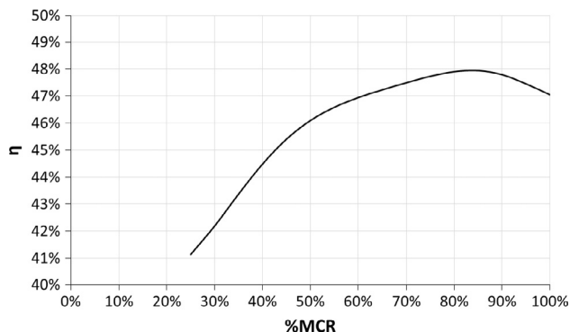
Fig. 7. Behavior of the engine efficiency vs. load % for the Wärtsilä #46C internal combustion engine, at fixed RPM. Data obtained from [42].
