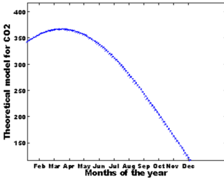
Figure 7: Theoretical model describing the CO 2 pattern and corresponding constants
