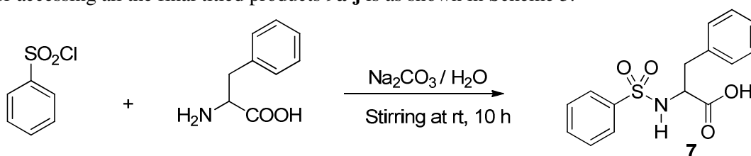
Scheme-1: Pathway for the synthesis of 3-phenyl-2-(phenyl sulfonamide)propanoic acid, 7
