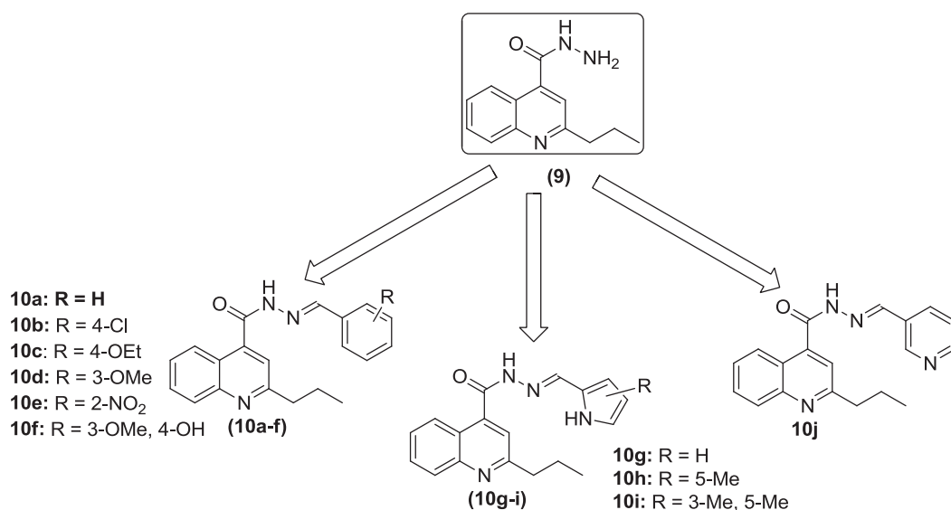
Regents: (a) benzaldehyde (b) 4-chlorobenzaldehyde (c) 4-ethoxybenzaldehyde (d) 3-methoxybenzaldehyde (e) 2-nitrobenzaldehyde (f) vanillin (g) pyrrole-2-carboxaldehyde (h) 5-methylpyrrole-2-carboxaldehyde (i) 3,5-dimethylpyrrole-2-carboxaldehyde (j) nicotinaldehyde. Reaction Condition: MW, Ethanol, for 1-3 min, 140 °C
