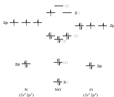
Figure 1. Molecular orbital energy level diagram for NO (Burrow et al., 2013)
