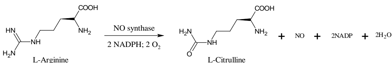
Figure 2. Synthesis of NO through the conversion of L-arginine to L-citrulline
