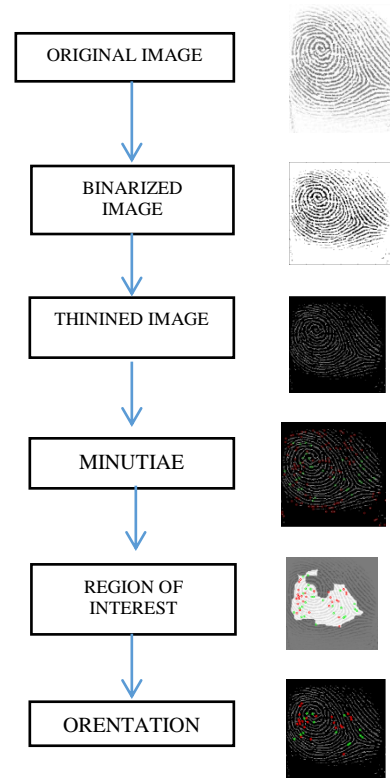
Fig. 3. Fingerprint extraction
