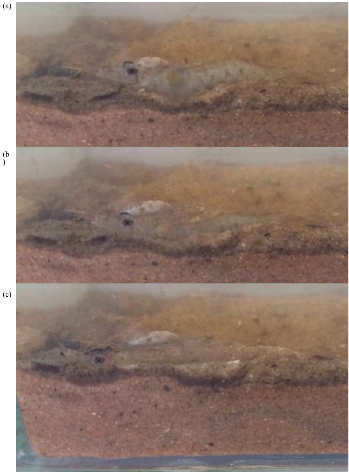
Fig. 1.8.12. Still frames of the burial process of Metapenaeus dalli in the laboratory at (a) 0, (b) 2 and (c) 8 seconds and by 17 seconds the prawn is completely buried.
