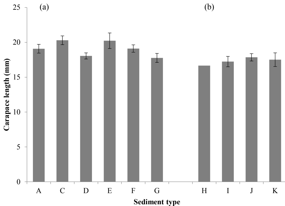
Fig. 1.8.6. The average carapace length (CL) of Metapenaeus dalli recorded at each of the sediment types present in the (a) offshore and (b) offshore waters of the Swan-Canning Estuary in summer ( i.e. November 2013-March 2014). Error bars represent \pm 1 standard error. Note sediment H has no error bar as only a single individual was recorded. Sediment types A to G were from the offshore waters with matching carapace length data from otter trawls, while those from H to K were in nearshore waters with CL data from hand trawls.
