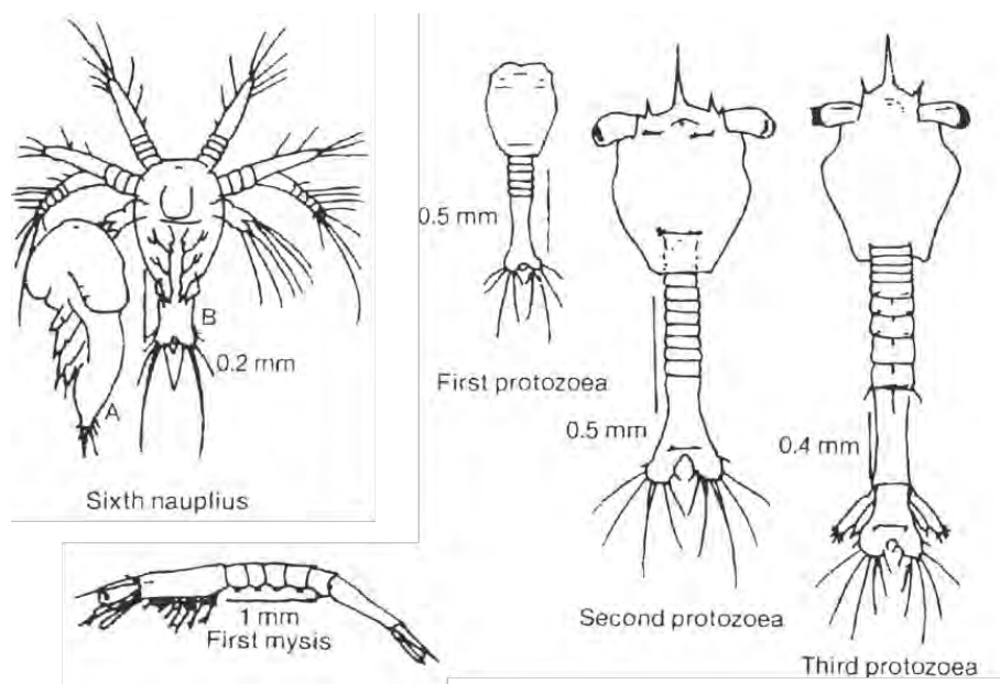
Fig. 1.6.1. Representation of the larval life-cycle of penaeid and metapenaeid prawns from nauplii sub-stage VI, through protozoa sub-stages I to III and on to mysis sub-stages I. Modified from: Motoh (1985).
