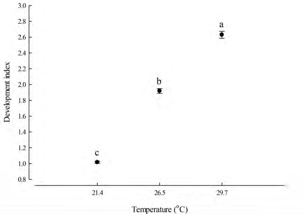
Fig. 1.5.4. Mean development index ( \pm 95\% CL) of Metapenaeus dalli larvae over a 48 h period from N VI sub-stage at three different water temperatures. Letters above error bars denote groups of samples identified by Tukey's HSD.
