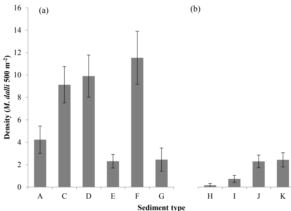
Fig. 1.8.4. The average density of Metapenaeus dalli (500m -2 ) recorded at each of the sediment types present in the (a) offshore and (b) nearshore waters of the Swan-Canning Estuary in summer ( i.e. November 2013-March 2014). Error bars represent \pm 1 standard error. Sediment types A to G were from the offshore waters with matching density data from otter trawls, while those from H to K were in nearshore waters with density data from hand trawls.
