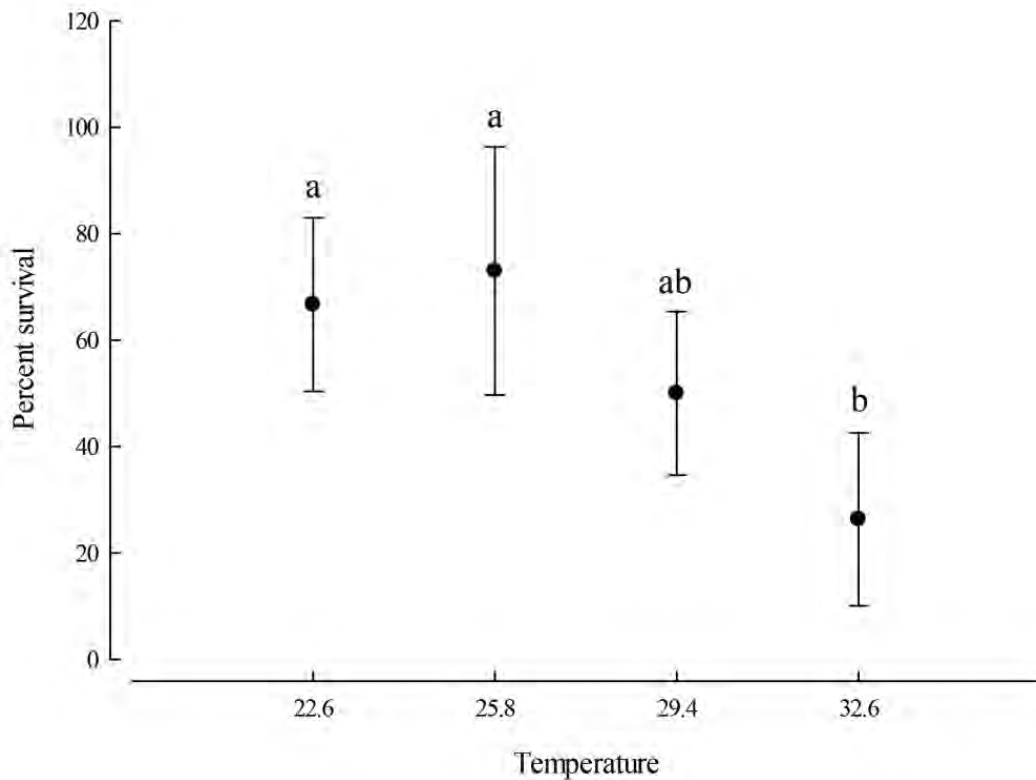
Fig. 1.5.1. Mean percentage survival ( \pm 95\% CL) of Metapenaeus dalli larvae during to development from Nauplius VI to Mysis I at four different water temperatures (in °C). Letters above error bars denote groups of samples identified by Tukey's HSD.
