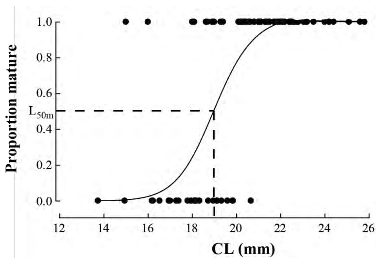
Fig. 1.3.4. Logistic regression curve of the carapace length at maturity of female Metapenaeus dalli collected from the Swan-Canning Estuary between October 2013 and January 2015. Dotted line represents the estimated CL at 50% maturity. N = 100. Females (black dots) with immature ovarian development were assigned a value of 0, while, late maturing, mature and post spawned females were assigned the value 1.
