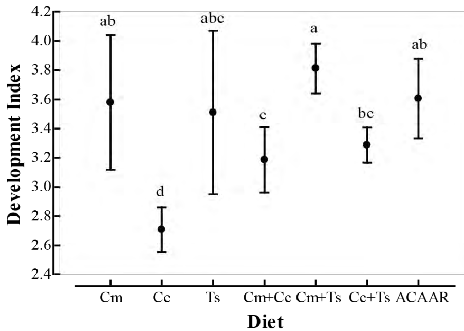
Fig. 1.6.3. Development of Metapenaeus dalli larvae (mean \pm 95% confidence limits; n=3 ) fed different algal diets determined at the time when 50 % the control (Cm+Ts) had moulted to M I. Chaetoceros muelleri (Cm), Chaetoceros calcitrans (Cc), Tetraselmis suecica (Ts), Australian Centre for Applied Aquaculture Research (ACAAR) = Cm +Cc+Ts. Bars with the same lower case letters denote groups that are not significantly different.
