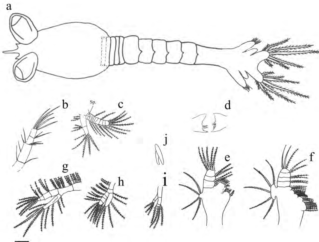
Fig. 1.4.10. Metapenaeus dalli Protozoea III dorsal view (a); (b) 1st antenna; (c) 2nd antenna; (d) mandible; (e) 1st maxilla; (f) 2nd maxilla; (g) 1st maxilliped; (h) 2nd maxilliped; (i) 3rd maxilliped; (j) pereiopod. Scale bar (a-c, g-i) = 0.1 mm, (d-f) = 0.05 mm.
