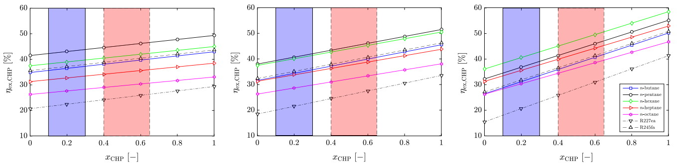
Fig. 3. CHP exergy efficiency of the ORC-CHP system as a function of the heat-demand intensity (coefficient x_{CHP} in Eq. (15)) for selected single-component working fluids, the high-temperature ( T_{hs} = 330\text{ }^{\circ}\text{C} ) heat source and hot-water supply temperatures of 45 °C (left), 60 °C (center) and 90 °C (right). The solid/blue and dashed/red areas represent the x_{CHP} ranges of residential and industrial heat demands, respectively. (For interpretation of the references to colour in this figure legend, the reader is referred to the web version of this article.)
