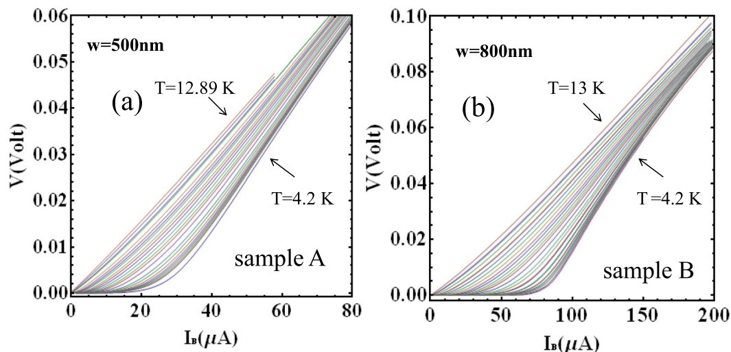
Figure 2. Current voltage characteristics: (a) Sample A, w = 500 nm. (b) Sample B, w = 800 nm for different temperatures between 4.2 K and 13 K. Sample A: ( T (K) = 4.2, 4.88, 4.97, 5.1, 5.29, 5.45, 5.72, 6.11, 6.38, 6.89, 7.31, 7.58, 7.88, 8.21, 8.5, 8.81, 9.19, 9.42, 9.74, 10.15, 10.96, 11.19, 11.84, 12.89). Sample B: ( T (K) = 4.2, 4.61, 4.78, 5.0, 5.33, 5.42, 5.86, 5.99, 6.46, 6.54, 6.99, 7.35, 7.83, 8.29, 8.53, 8.81, 9.12, 9.44, 9.82, 10.2, 10.62, 11.06, 11.13, 11.63, 12.16, 12.29, 13.0).
