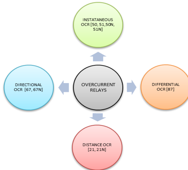
Figure 1.1 Overcurrent relay classification
