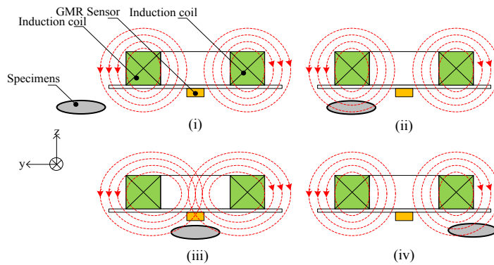
Figure 1. The application of MFLT method where (i) condition before evaluation, (ii) specimen navigates into the system, (iii) the magnetic flux distribution changes according to the disturbance and (iv) system fully evaluates the specimen
