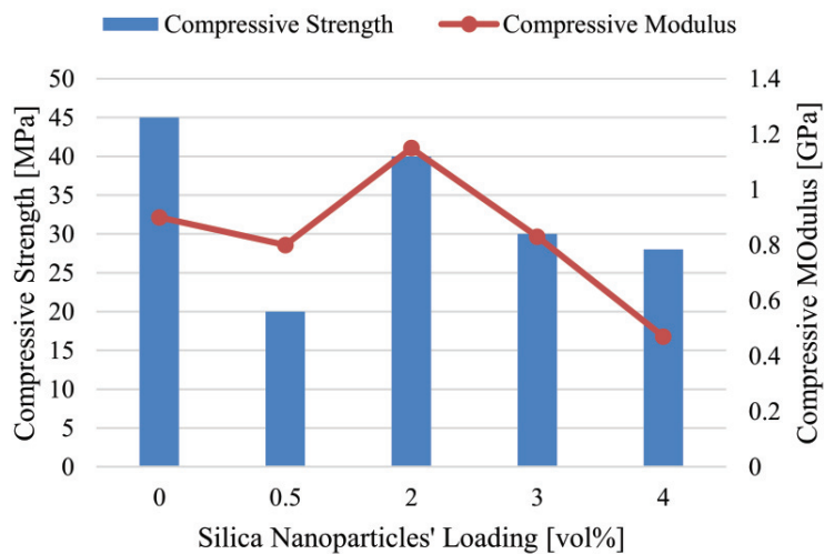
Fig. 3. Compressive properties of fabricated specimens
