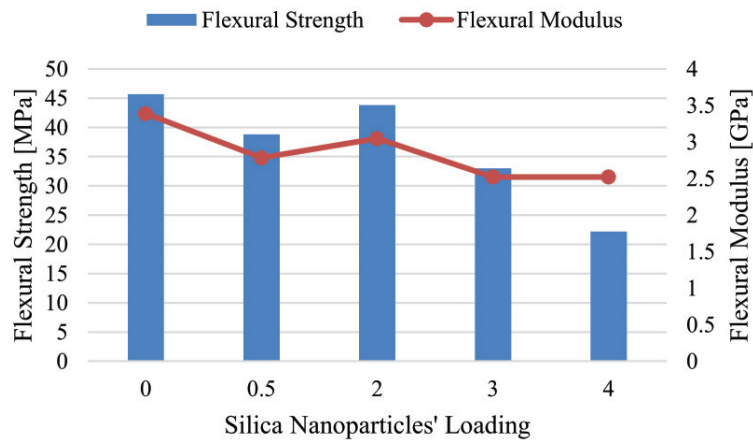
Fig. 2. Flexural properties of fabricated specimens
