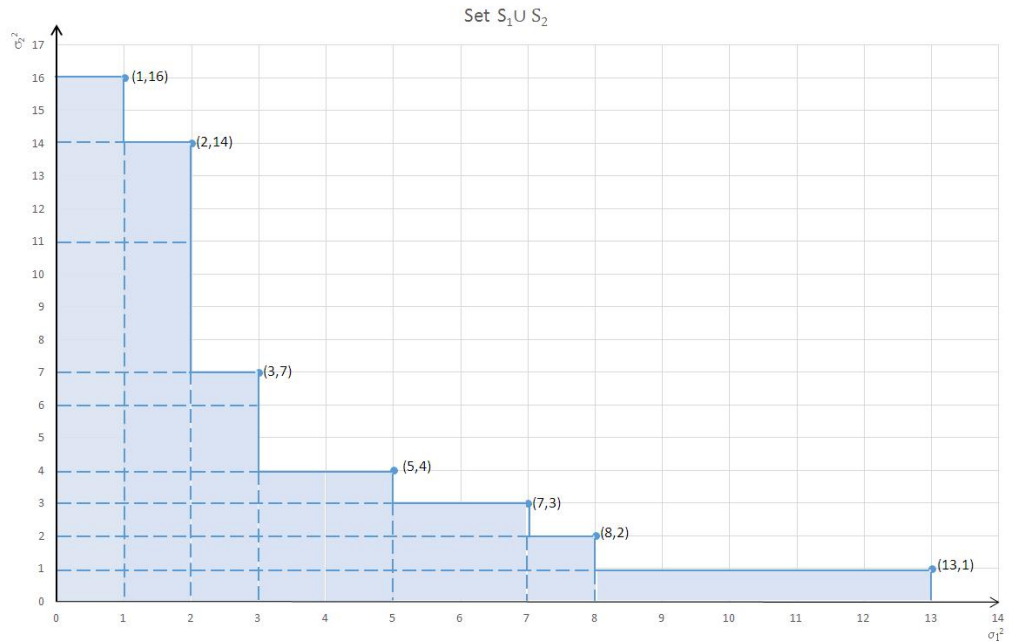
Figure 1: The set S corresponding to the pursuers' resources (\rho_{11}^2, \rho_{12}^2) = (1, 2) , (\rho_{21}^2, \rho_{22}^2) = (2, 3) , (\rho_{31}^2, \rho_{32}^2) = (2, 4) , (\rho_{41}^2, \rho_{42}^2) = (3, 6) , (\rho_{51}^2, \rho_{52}^2) = (5, 1) .
