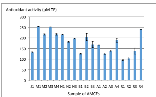
Figure 3. Oxygen radical absorbance capacity (ORAC) assay for 19 samples of Annona muricata crude extract equivalent to Trolox ( \mu\text{M} ). Each value is expressed as the mean from three replicate measurements. The error bars indicate standard deviations
