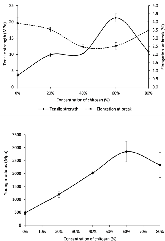
Figure 1. Effect of chitosan concentrations on tapioca starch film (a) tensile strength and elongation at break, (b) young modulus
