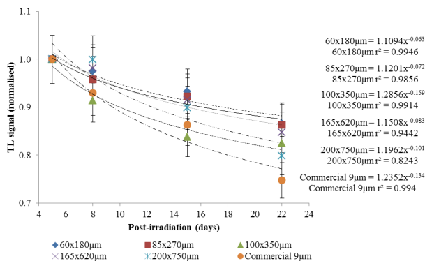
Figure 4. Post-irradiation of fading for fabricated Ge-doped flat fibres and also commercial fibres under normal ambient conditions
