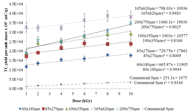
Figure 2. Linearity of the Ge-doped flat fibres and commercial fibres for kiloGray gamma irradiation
