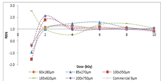
Figure 3. Linearity index of optical fibres
