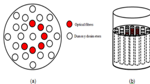
Figure 1. (a) The top view of Gammacell chamber with samples and dummy dosimeters. (b) The side view of Gammacell chamber
