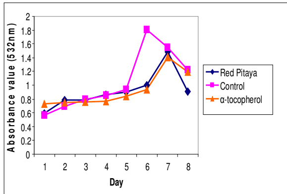
Figure 1. Absorbance value of red pitaya extract (4.0 mg/ml concentration) using FTC method. The values are compared with the absorbance values of the control and \alpha -tocopherol at 532 nm. Each value represents the mean of three replications and betaxanthins (Wybraniec et al. , 2001). Anthocyanin is the antioxidant component which involved giving the red, blue and indigo colour pigment to the fruits (Wang et al. , 1997). Highest content of anthocyanin also reflect the highest present of phenolics content in the fruits and vegetables, which anthocyanin is the phenolics component which existing in human diet (Javanmardi et al. , 2003).
