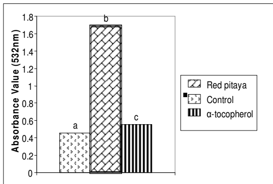
Figure 2. Total antioxidant activity of methanolic extract of red pitaya, \alpha -tocopherol and control using TBA method. Value represents the mean of three replications
