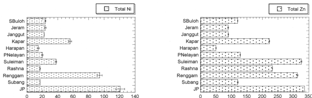
Fig. 2: Total concentrations (mean \text{mg/g} \pm \text{SE} dry weight) of Ni and Zn in surface sediments collected from Tanjung Harapan to Sungai Buloh, based on direct aqua-regia method
