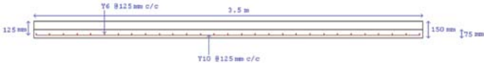
Fig. 14: Graphical representation of the composite slab
