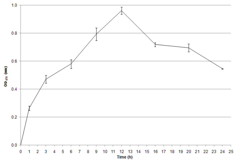
Figure 2. Mean value of biofilm formation by Salmonella Typhimurium on plastic cutting board represented by OD 570 . Each error bar represents the standard error of mean of triplicate measurements.
