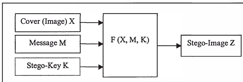
Figure 1.1: Steganographic Encoding
