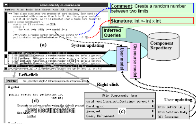
Figure 3.10: CodeBroker System [157]
