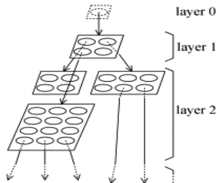
Figure 3.6: GHSOM Architecture [142]
