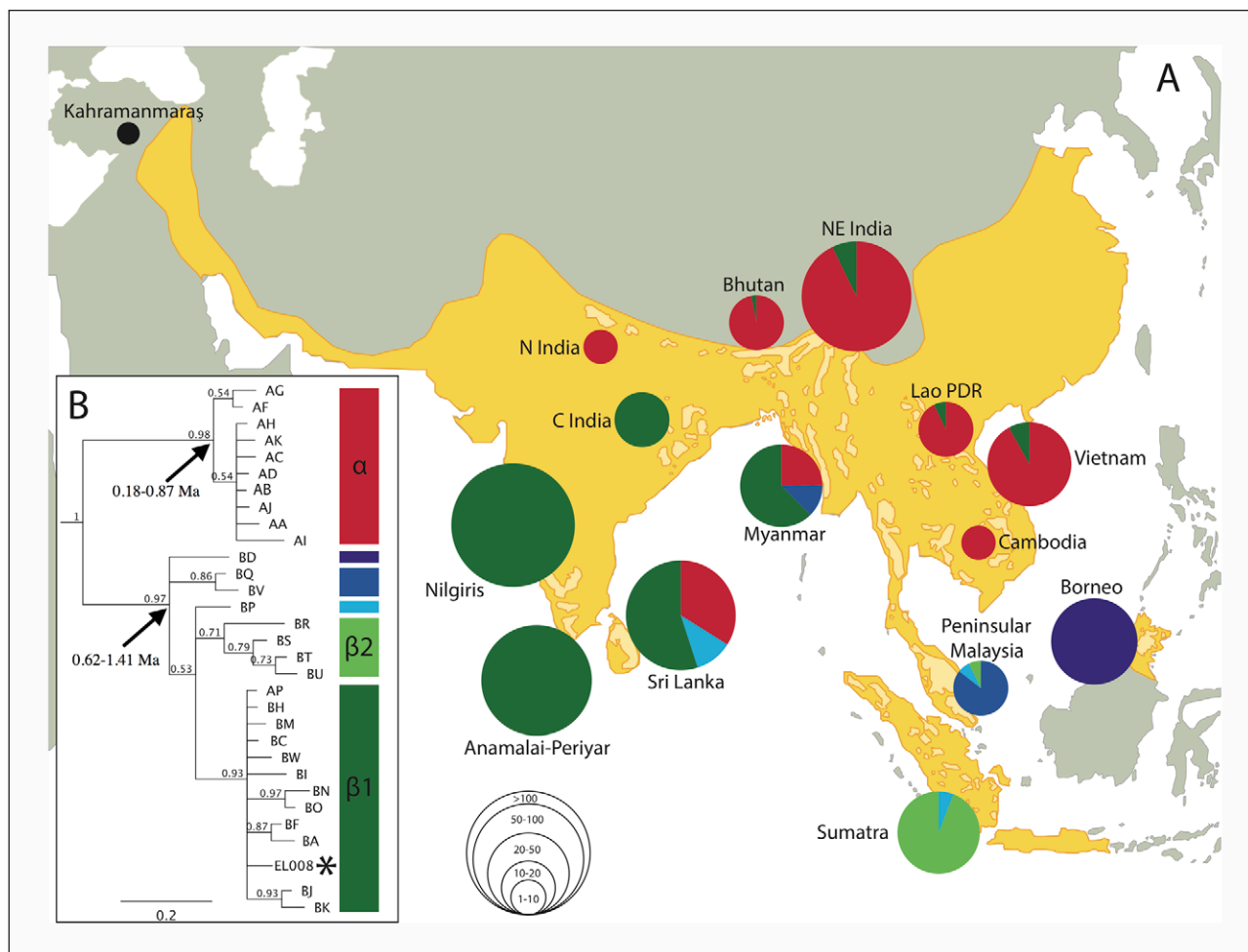
Figure 1: (A) A map depicting the present-day (light yellow) and ancient (dark yellow) range of Elephas maximus (Olivier 1978, Choudhury et al. 2008), the location of Kahramanmaraş, and the relative proportion of mtDNA haplotypes based on data published in Vidya, Sukumar and Melnick (2009). (B) A Bayesian phylogenetic tree produced in MrBayes of haplotypes analysed in Vidya, Sukumar and Melnick (2009), but restricted to the 570 base pairs sequenced for this study. Numbers show posterior support values for the nodes. Arrows indicate node age estimates (see Results). Nomenclature is reported as in Vidya, Sukumar and Melnick (2009). The asterisk denotes the haplotype observed in the Kahramanmaraş elephants, here represented by sample EL008 (Table 1).
