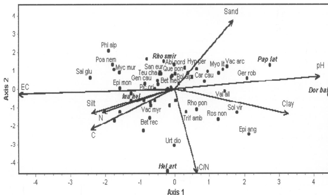
Fig. 2. The CCA ordination diagram showing the relationships between species and soil factors. For species codes see Table 1. C: N; N: nitrogen content; C/N: carbon to nitrogen ratio; Clay: proportion of clay; Sand: proportion of sand; Silt: proportion of silt; EC: electrical conductivity.
