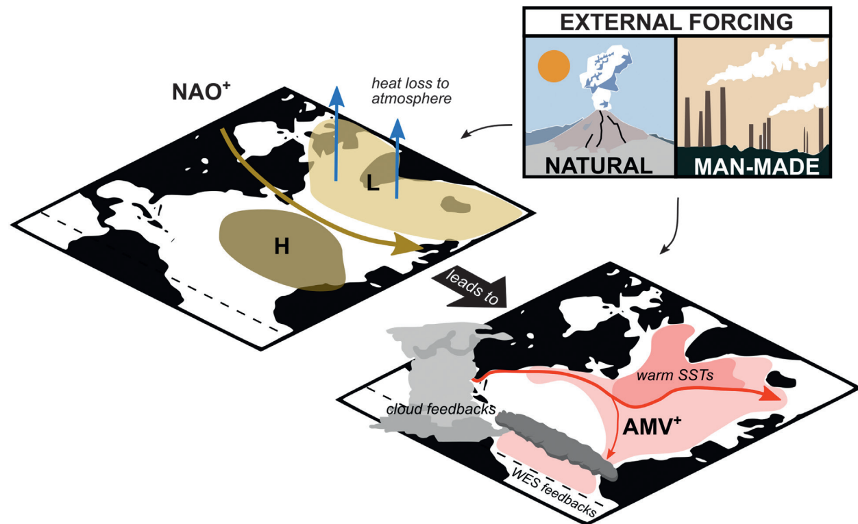
FIG. 2. Schematic illustrating processes involved in AMV. The left-hand map shows typical NAO + conditions with the Greenland low (~1,010 hPa) and the Azores high (~1,020 hPa) highlighted with the storm track illustrated between (brown arrow). NAO + conditions result in heat loss from ocean to the atmosphere, particularly over the Labrador and Irminger Seas (blue arrows), leading to deep convection and cool SSTs, itself indicative of AMV - . Increased deep convection is linked with increasing northward ocean heat transport (red arrows), associated with a strong AMOC, leading to warmer SSTs, indicative of AMV + , as shown in the right-hand map. External forcing from natural solar and volcanic variability and from manmade aerosols have been proposed as additional drivers of AMV. Ocean–atmosphere feedbacks are important in the amplification and modification of AMV patterns including interactions with tropical and subtropical clouds and WES interactions.
