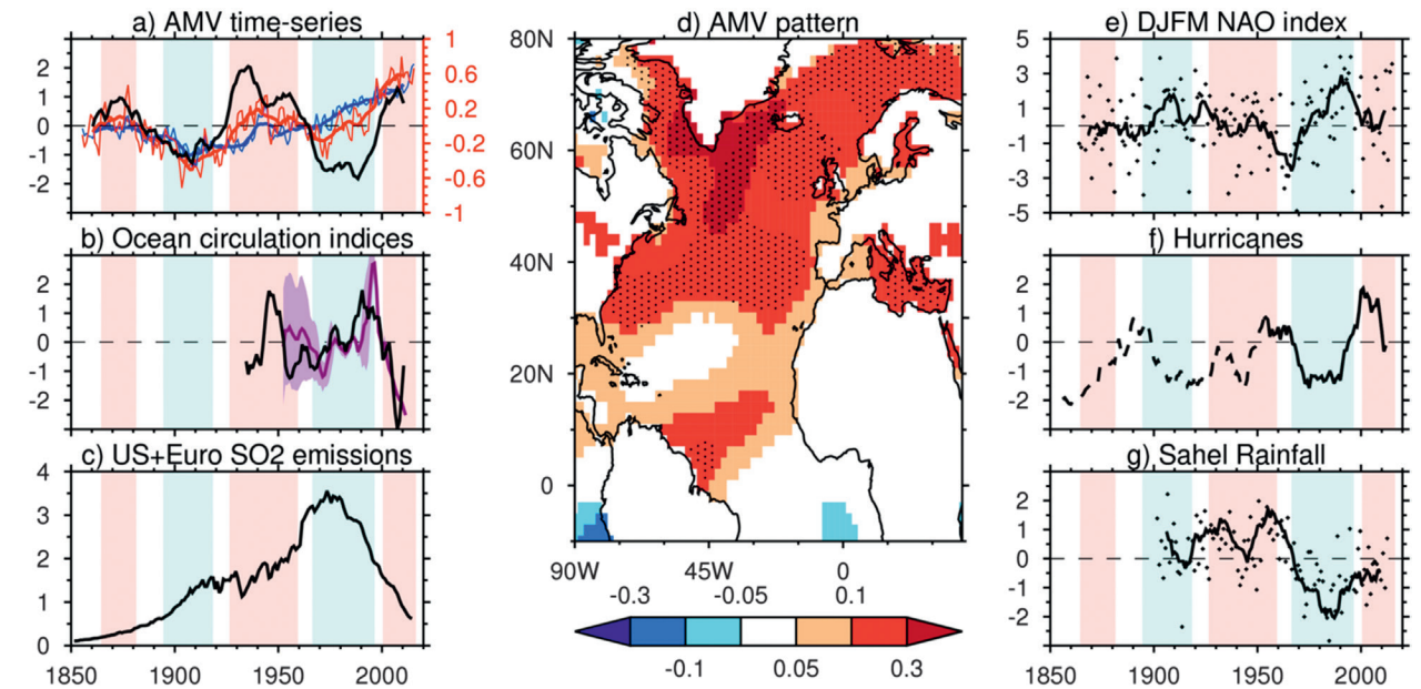
FIG. 1. (a) Atlantic-mean (0°–65°N, 75°–7.5°W) sea surface temperatures (red) and global mean excluding the North Atlantic (blue) sea surface temperatures for annual means (thin lines) and decadal mean (thick lines) based on the Extended Reconstructed SST, version 4 (ERSST.v4), dataset (Huang et al. 2015). Units are °C, and anomalies are made relative to the entire 1855–2016 period. The AMV index is shown in black, which is the normalized difference between the 10-yr smoothed Atlantic (red) and global-mean (blue) indices. This definition follows Sutton and Dong (2012) and is close to that of Trenberth and Shea (2006). Periods where the AMV index is larger than 0.5 or smaller than –0.5 are highlighted with red and blue filled sections, respectively. (b) Ocean circulation proxies, including the sea level dipole index (black) based on McCarthy et al. (2015a) and the 1,000–2,500-m Labrador Sea density index (purple) from Robson et al. (2014). Purple shading shows the 5%–95% confidence interval for the deep Labrador Sea density. (c) The emissions of SO 2 from the United States and Europe from the CMIP6 emissions dataset. (d) The SST pattern associated with the AMV index, represented by the regression slope between the AMV index in (a) and the annual-mean SST anomalies at each grid point over the period 1990–2016. Stippling is a measure of signal to noise and shows where the variance explained is >20% of the interannual variance at each grid point, after a linear trend has been removed. (e) The Dec–Mar (DJFM) NAO station index data (Hurrell et al. 2003); black dots show individual years, and the thick black line shows the 10-yr running mean. (f) The accumulated cyclone energy from 1948 to 2016 from the National Hurricane Center (NHC) “best track” hurricane database (HURDAT) (solid; Landsea et al. 2004) and from 1851 to present (dashed). (g) JJAS rainfall anomalies over the Sahel (10°–20°N, 20°W–40°E) from the GPCP dataset (Schamm et al. 2014); dots show the annual means and the black curve shows the 10-yr running mean. All time series are normalized by their standard deviation, apart from the blue and red curves in (a).
