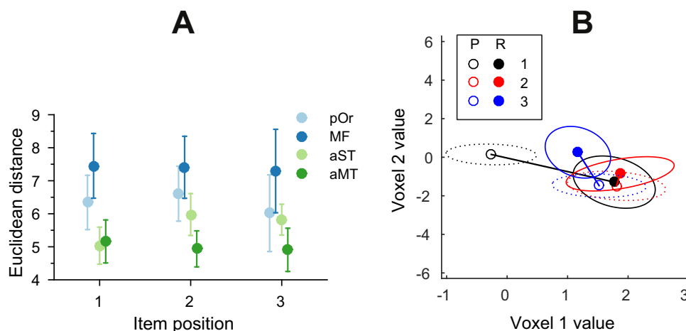
Fig. 5. (A) Change in position representations across task phases averaged over participants in prefrontal (blue) and temporal (green) regions of interest. Error bars show the standard error of the mean. Analysis of variance was significant for region ( F=10.38 , df=3 , p < 0.001 ) but not position ( F=0.23 , df=2 , p=0.79 ). (B) Change in position representations for a single subject between two task phases. For visualisation purposes only values from two most discriminant voxels are plotted. Empty markers represent the distribution of means for the presentation phase, filled markers for the recognition phase. Black – first position, red – second position, blue – third position. Ellipses represent two standard deviations around the mean: dotted ellipses – presentation, solid ellipses – recognition. Straight lines represent the Euclidean distance the mean of the distribution has moved in two-voxel space between presentation and recognition.
