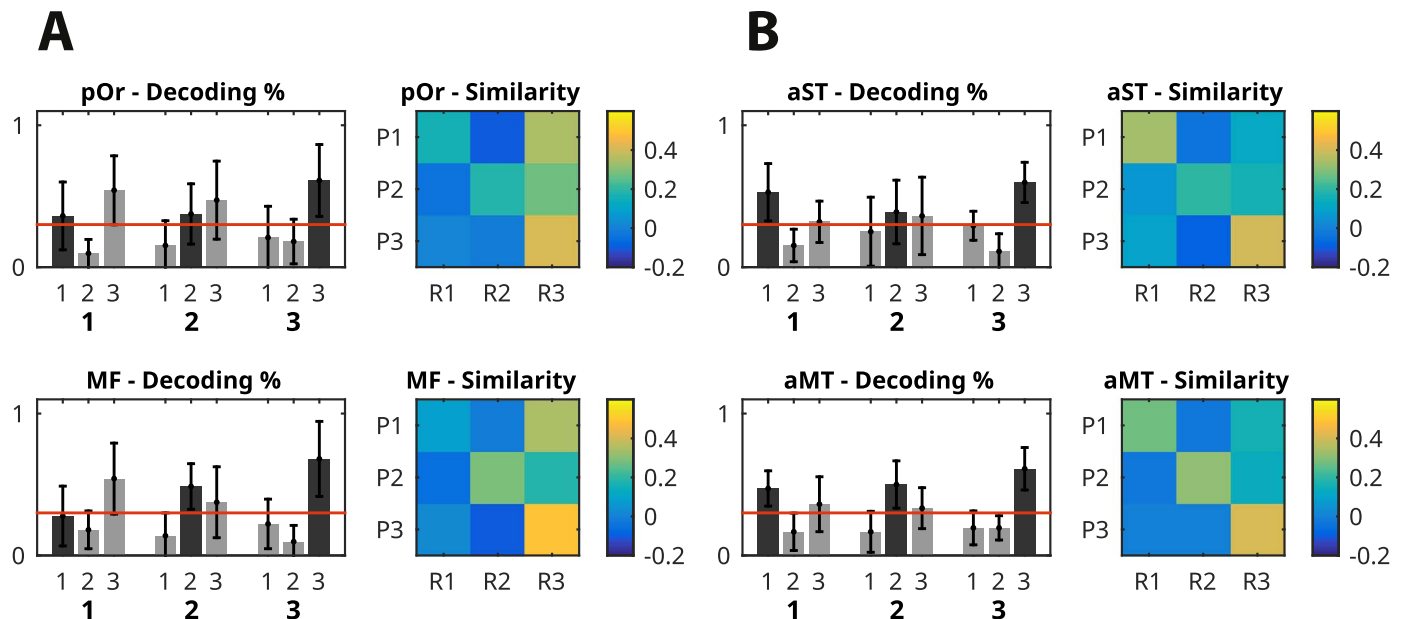
Fig. 4. Classification accuracy and pattern similarity between two task phases in rostro-lateral prefrontal (A) and anterior temporal regions (B). Bar charts display the average classification accuracy across participants by comparing the known position labels (bar groups) to the predictions made by the classification algorithm (bars within the group). Bars show the proportion of predicted values for each position. Correct classifications are represented with a darker bar. Error bars show the standard error of the mean. The red line depicts the chance level classification accuracy 1/3. Similarity matrices display average pairwise pattern correlations (Pearson’s \rho ) between two task phases: P – presentation, R – recognition, 1, 2, 3 – position. Cells on the diagonal show the pattern correlation within the same positions between two task phases. Abbreviations: MF – middle frontal lobe, pOr – pars orbitalis, aST – antero-superior temporal lobe, aMT – anterior middle temporal lobe.
