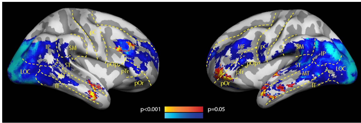
Fig. 3. Regions where the position of the items within a sequence was decoded significantly above chance across participants: red-yellow – significantly above chance between task phases, blue-cyan – significantly above chance within a presentation task phase only. Note that within-phase and across-phase classification maps are not directly comparable and are overlaid here only for visualisation purposes (see Supplementary Information ‘Item position classification accuracy within single task phases’ for more information). Abbreviations correspond to the following cortices: MF – middle frontal lobe, pOr – pars orbitalis, pTr – pars triangularis, pOp – pars opercularis, pC – precentral area, ST – superior temporal lobe, MT – middle temporal lobe, IT – inferior temporal lobe, LOC – lateral occipital lobe, SM – supramarginal area.
