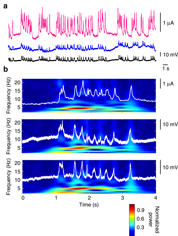
Figure 4 | Validation in GAERS rats. (a) Recordings from an OECT (pink), a PEDOT:PSS surface electrode (blue) and an Ir-penetrating electrode (black). The transistor was biased with V_D = -0.4 V and V_G = 0.3 V, and the scale of 10 mV is for both surface and penetrating electrodes. Note the superior SNR of the OECT as compared with the surface electrode. (b) Time–frequency analysis of epileptiform activity during a short period, recorded by an OECT (top), a PEDOT:PSS surface electrode (middle) and an Ir-penetrating electrode (bottom).
