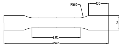
Fig. 1 Tensile and fatigue sample dimensions (in mm) according to EN-BS 895:1995 and BS 7270 standards [5]
