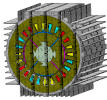
Fig. 5. The magnetic-thermal coupling finite element model of SIPMSM.
