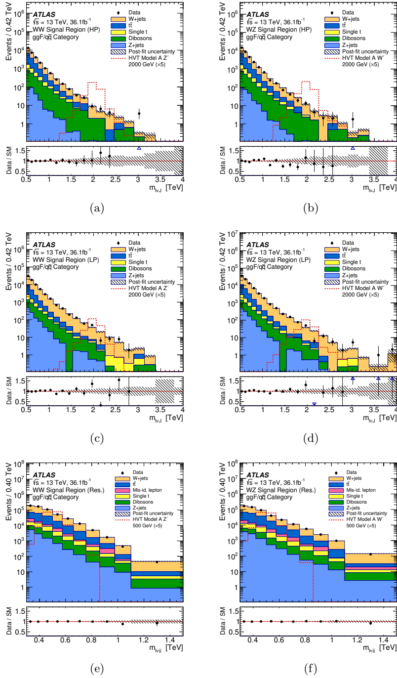
Figure 5. Post-fit signal region m(WV) distributions in the ggF/ q\bar{q} category. The merged high-purity (HP) sample of (a) WW and (b) WZ events, the merged low-purity (LP) sample of (c) WW and (d) WZ events and the resolved (Res.) sample of (e) WW and (f) WZ events are presented. The expected background is shown after the profile likelihood fit to the data, and signal predictions are overlaid. The HVT Model A signal at 2000 GeV is presented for the merged analysis, while the 500 GeV signal is shown in the resolved topology. The band denotes the statistical and systematic uncertainty in the background after the fit to the data. The lower panels show the ratio of the observed data to the estimated SM background. The distribution of events is shown per mass interval corresponding to the penultimate bin width, while the overflow events are included in the last bin.
