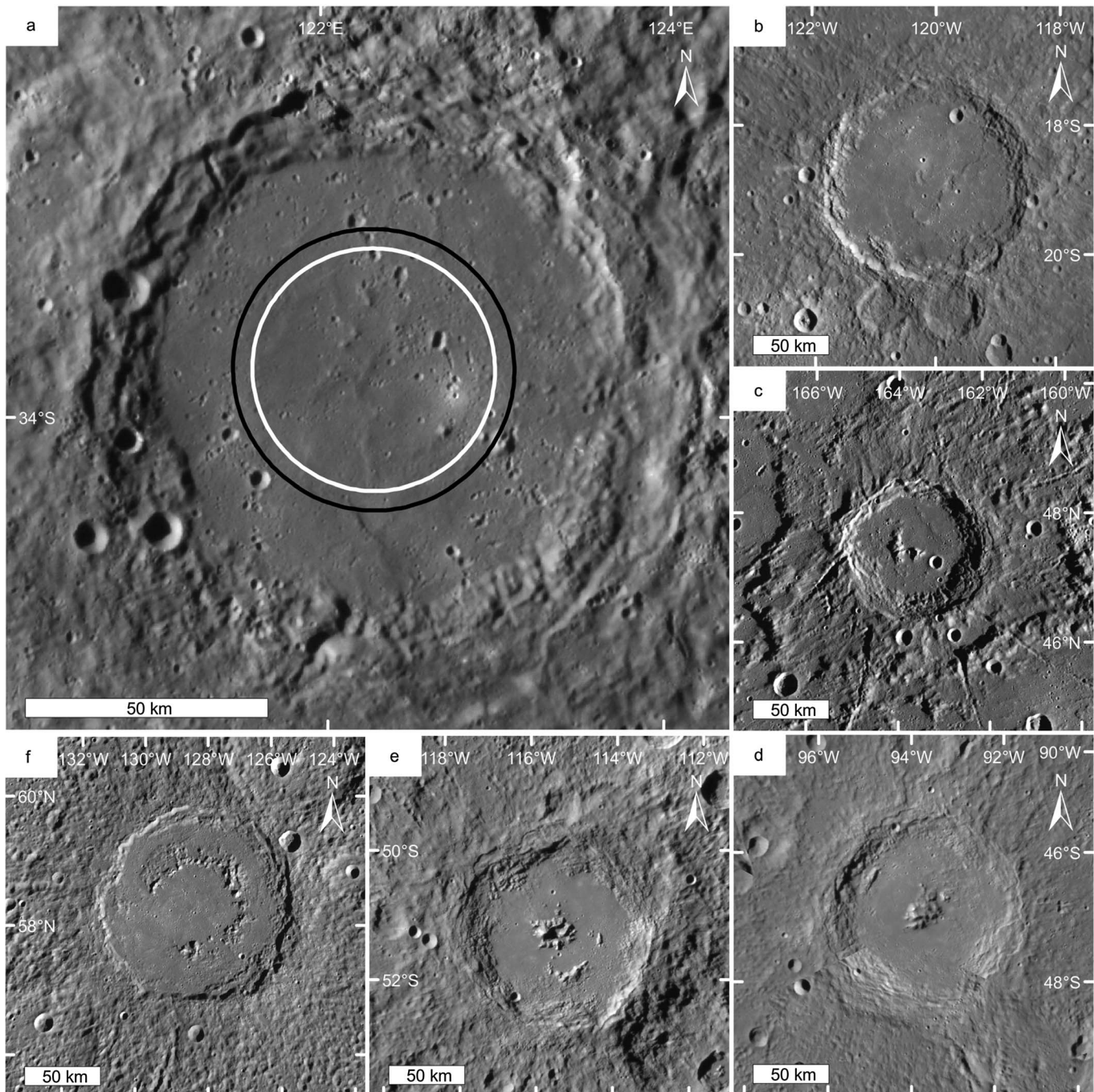
Figure 3. Comparison of Heaney with other impact features on Mercury that are similar in age and size. (a) Heaney. The circles represent expected radii of peak-rings (black) and protobasin (white) of similar diameter to Heaney, per equation (2). Note that the other small knobs in Heaney do not lie where one would expect to find the highest peak elements. (b) Bello (diameter 139 km) located within Beethoven. Bello has a very similar size, apparent morphology, and degradation state to Heaney. Smooth plains, of probable volcanic origin, obscure any internal peaks that may have been present. (c) Mansur (diameter 95 km), the degradation state of which defines the base of the Mansurian time system on Mercury. Heaney has a similar degradation state, suggesting that it formed at a similar time. (d) Sūr Dās (diameter 131 km) with a central peak rather than a peak-ring. It is therefore possible that Heaney originally had no peak-ring. (e) Hawthorne (diameter 120 km), a protobasin. (f) Ahmad Baba (diameter 126 km), a peak-ring basin.
