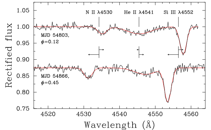
Fig. 7. VFTS 652 as a double-lined spectroscopic binary (Sect. 4.3). Wavelengths of selected lines are shown in the rest frame of the system centre of mass, together with the observed orbital displacements of N II \lambda 4530 , Si III \lambda 4552 (primary spectrum), and He II \lambda 4541 (secondary spectrum).
