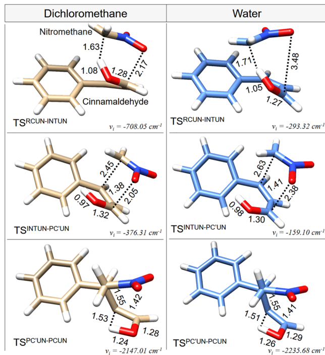
Figure 6. Representation of the TS structures obtained along the reaction coordinate of the uncatalyzed Michael addition of nitromethane to cinnamaldehyde in DCM and in water. Key interatomic distances are reported in Å, while imaginary frequencies are reported in cm -1 .
