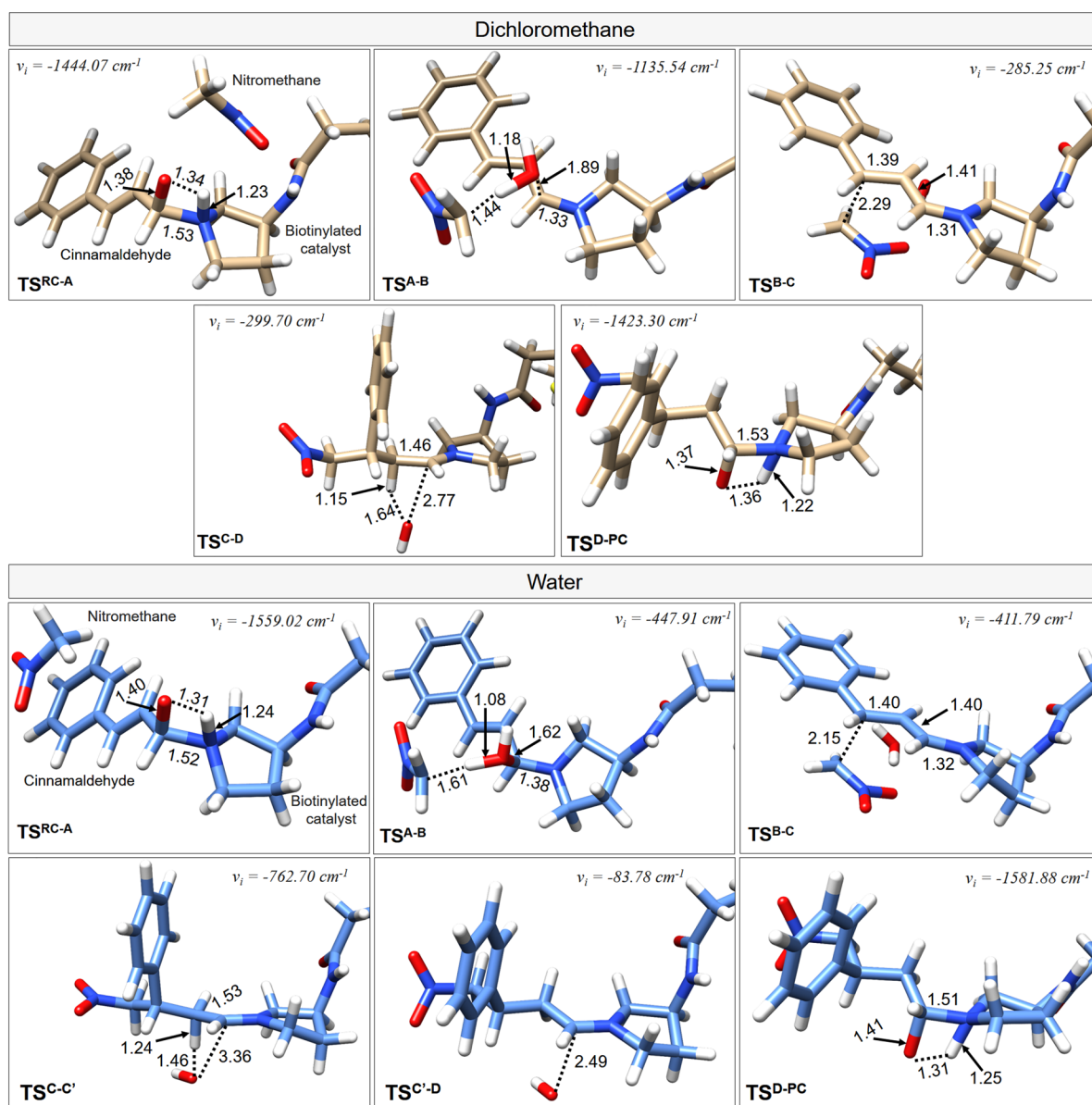
Figure 3. Representation of the TS structures obtained along the reaction coordinate of the catalyzed Michael addition of nitromethane to cinnamaldehyde in DCM and in water. Key interatomic distances are reported in Å, while imaginary frequencies are reported in \text{cm}^{-1} .
