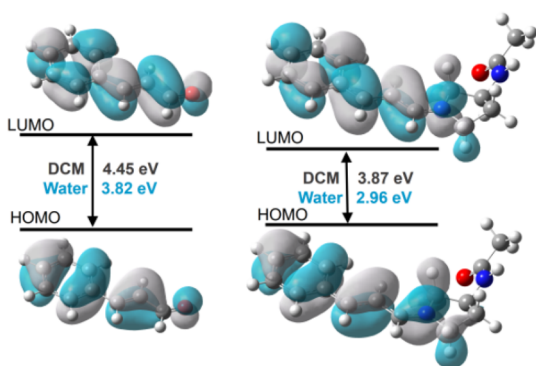
Figure 7. Frontier orbital representation of isolated cinnamaldehyde (left) and the iminium intermediate, INT-B (right). Results computed with TDDFT at the M06-2X/6-31G(d,p) level in DCM and in water.
