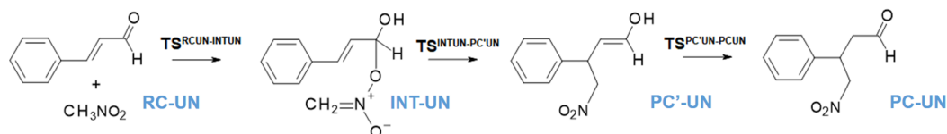
Figure 4. Schematic representation of the reaction mechanism of the noncatalyzed Michael addition of nitromethane to cinnamaldehyde in DCM.
