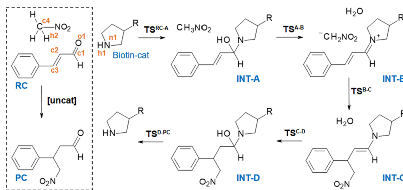
Figure 1. Schematic representation of the reactants complex (RC), products complex (PC), and intermediate states located along the catalyzed Michael addition of nitromethane to cinnamaldehyde in DCM. R = NH-biotin. The direct noncatalyzed reaction from RC to PC is indicated in the dashed rectangle. Labels of key atoms are shown in the RC panel.
