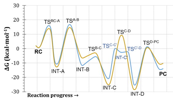
Figure 2. M06-2X/6-31+G(d,p) free energy profiles for the catalyzed Michael addition of nitromethane to cinnamaldehyde obtained in DCM (orange line) and in aqueous solution (blue line).
