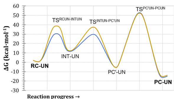
Figure 5. Free energy profile for the uncatalyzed Michael addition of nitromethane to cinnamaldehyde obtained in DCM (orange line) and in aqueous solution (blue line).
