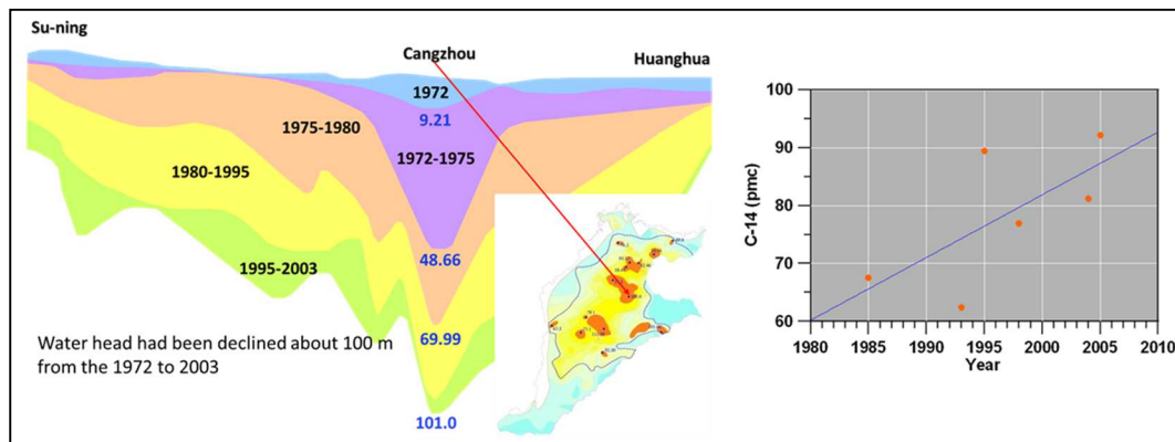
Figure 1: Dramatic changes of depression cones in Cangzhou, China. Increasing ^{14}\text{C} activity with groundwater exploitation indicates a short turnover time of the local groundwater system after the intensive groundwater abstraction
