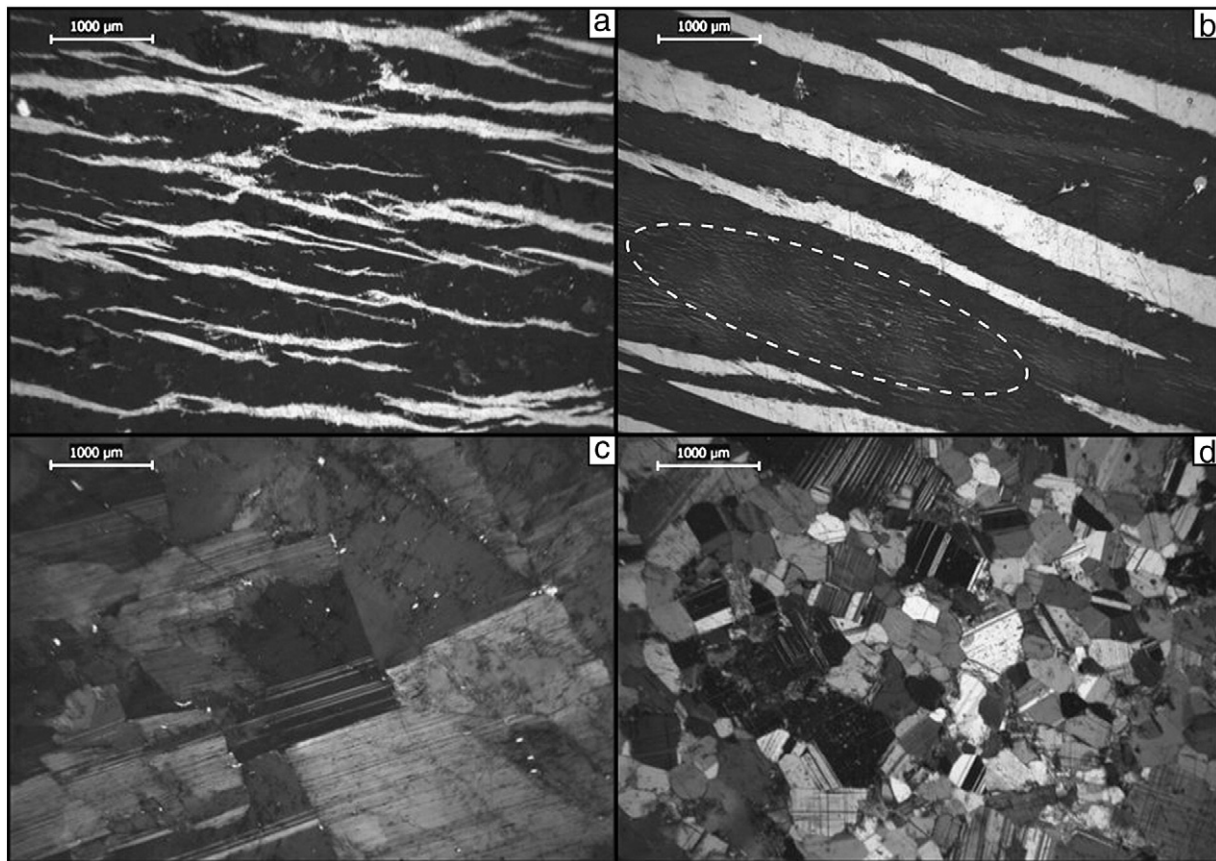
Fig. 2. Photomicrographs under crossed nichols. a) LSR1 sample: It shows development of lamellar perthites with irregular boundaries; b) FB sample: It shows development of lamellar lenticular perthites with net boundaries and spindle-like ends. An area where smaller grain size perthites have developed is enclosed in a dotted line; c) LSR3 sample: It shows intergrown crystals of plagioclase with straight boundaries; and d) AN sample: Plagioclase crystals arranged in a polygonal mosaic.
