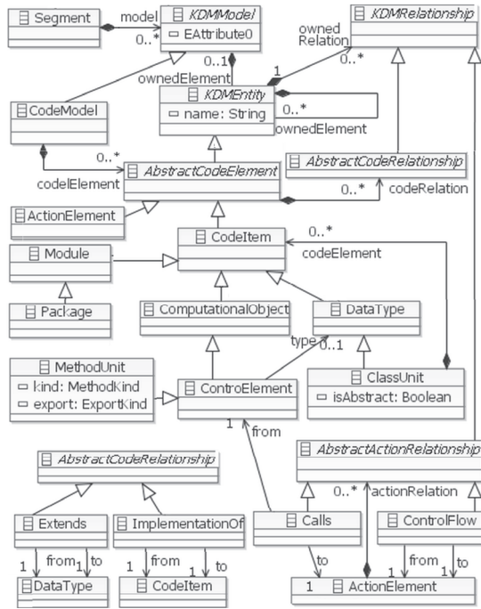
Figure 3: KDM metamodel.
