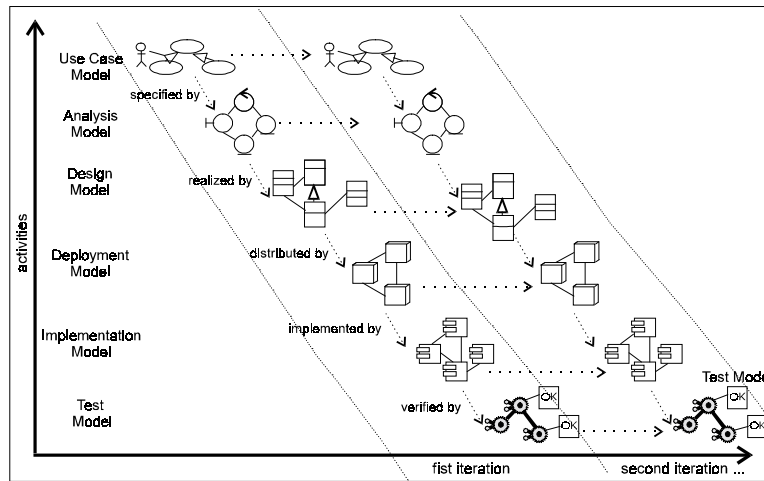
Figure 1. dimensions in the software development process
