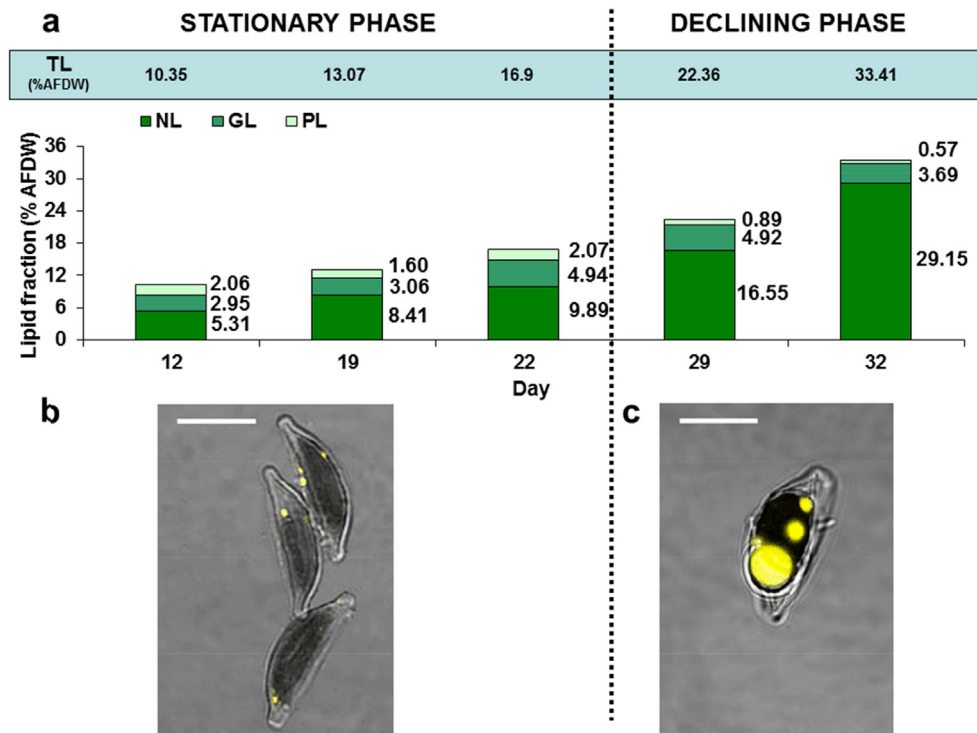
Fig. 3. Halamphora coffeaeformis ' lipid accumulation in stationary and declining phases. a. Total lipid content (TL) as a percentage of ash-free dry weight biomass (% AFDW) and lipid fractions (in % AFDW). Neutral lipids (NL), glycolipids (GL) and phospholipids (PL). b-c. Nile Red stained cells showing neutral lipid droplets in stationary and declining phases, respectively. Scale bars: 20 \mu\text{m} .
