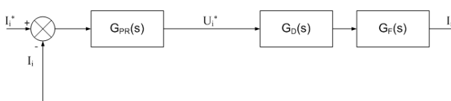
Fig. 3 The PR Current Control
