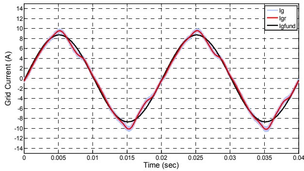
Fig. 15 Grid Current with PI Current Control
