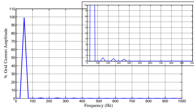
Fig. 13 Simulation Grid Current Harmonic Spectrum with PR Current Control with Harmonic Compensation
