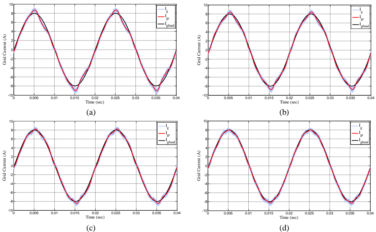
Fig. 16 Grid Current with PR Current Control a) without Harmonic Compensation, b) with 3 rd Harmonic Compensator, c) with 3 rd and 5 th Harmonic Compensators, d) with 3 rd , 5 th and 7 th Harmonic Compensators
