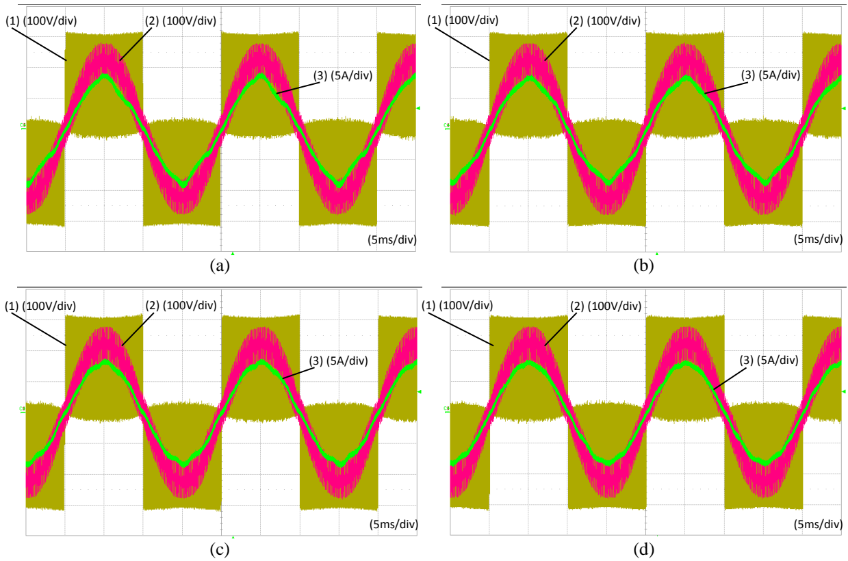
Fig. 15 Inverter Output Voltage (1), Grid Voltage (2) and Grid Current (3) with a Preset Current of 8A Peak using a) the PR Controller without Harmonic Compensation, b) the PR Controller with 3 rd Harmonic Compensation, c) the PR Controller with 3 rd and 5 th Harmonic Compensation, d) the PR Controller with 3 rd , 5 th and 7 th Harmonic Compensation
