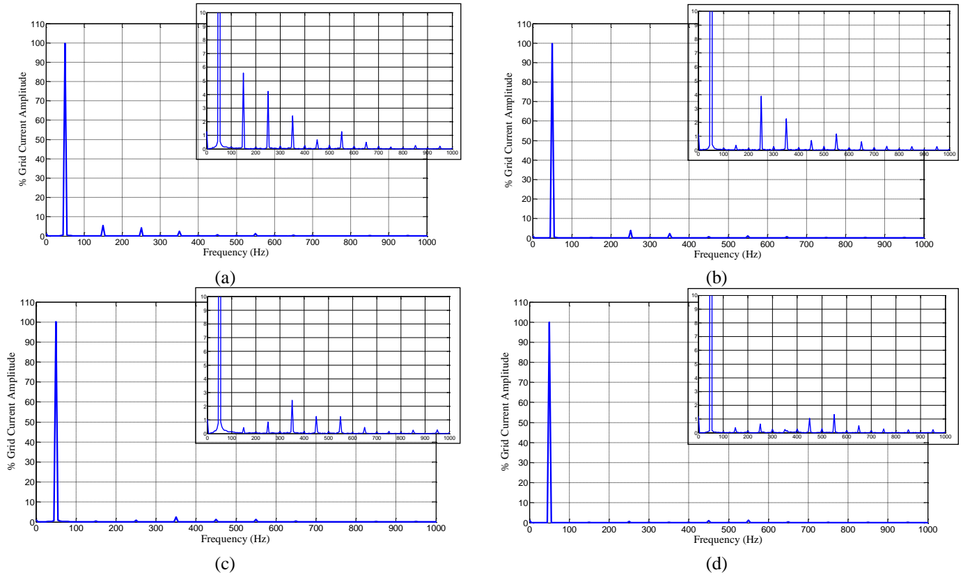
Fig. 17 Harmonic Spectrum of the Grid Current with PR Current Control a) without Harmonic Compensation, b) with the 3 rd Harmonic Compensator, c) with the 3 rd and 5 th Harmonic Compensators, d) with the 3 rd , 5 th and 7 th Harmonic Compensators
