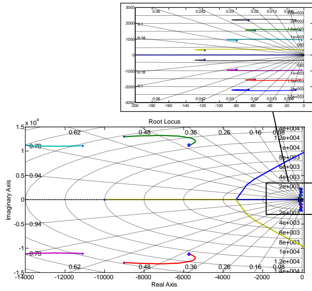
Fig. 7 Root Locus of the Inverter with the Fundamental PR Controller and the Harmonic Compensators
