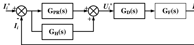
Fig. 3 The PR Current Control with Harmonic Compensators
