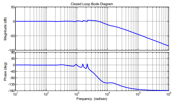
Fig. 9 Closed Loop Bode Diagram of the System with the Fundamental PR Controller and the Harmonic Compensators
