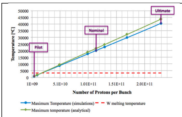
Figure 5: Variation in maximum temperatures reached with different proton populations (at 7TeV, 0mrad case).
