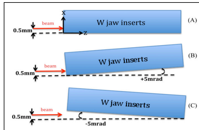
Figure 1: Schematic diagram of the studied accident scenarios. (A) Ideal case: perfect alignment of jaw with beam direction (0mrad angle). (B) & (C) Cases with jaw inclination due to misalignment errors.
