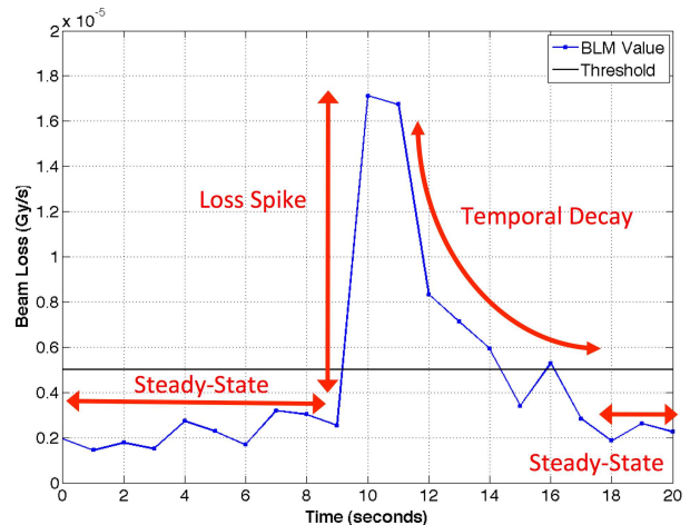
Figure 1: The components of a typical clear BLM signal when the collimator jaw touches the beam halo.
