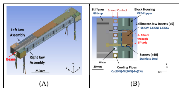
Figure 1: A horizontal tertiary collimator (TCTH). (A) 3D model. (B) Detailed cross-section in the x-y plane of the left jaw assembly.
