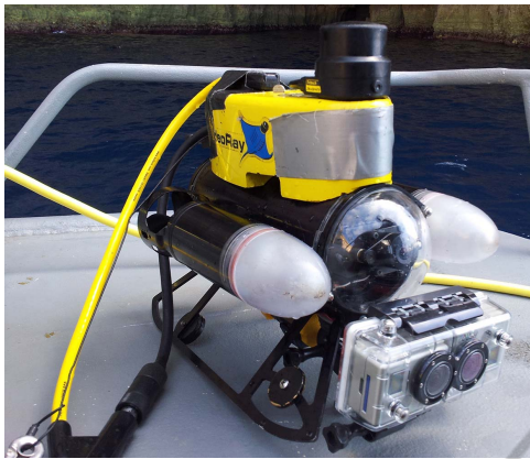
Figure 2: The VideoRay Pro III GTO is an underwater micro-ROV (36.8 cm x 28.9 cm x 21.6 cm), with a depth sensor, a compass, and a front and rear video camera. A removable Tritech Micron scanning sonar was mounted to the top and two vertically aligned GoPro Hero2 cameras were mounted to the front in a waterproof stereo casing.
