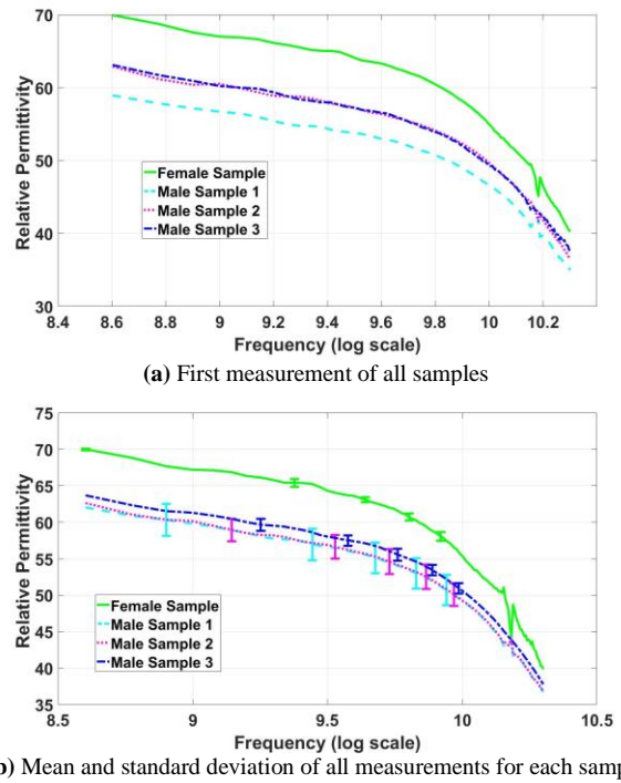
Figure 5. Real part of complex permittivity of blood with sodium citrate a) first measurement of all samples and b) mean and standard deviation over all measurement times.
