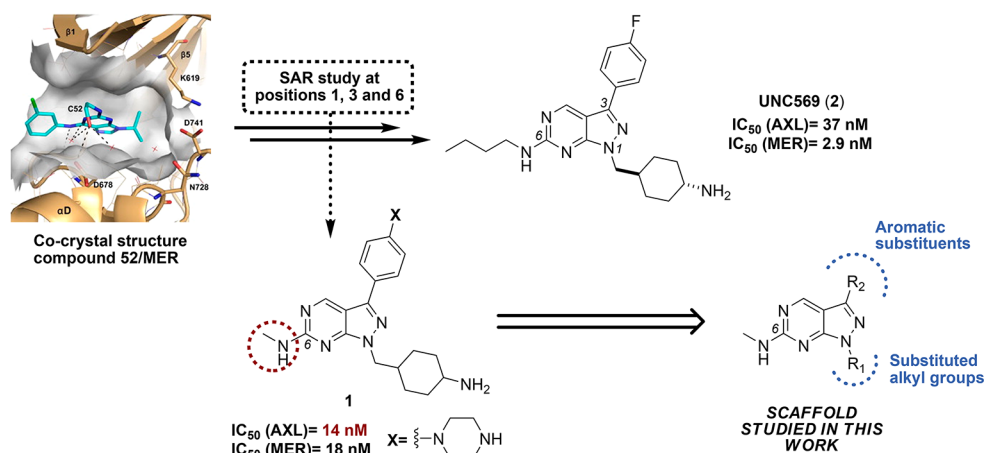
Figure 1. Medicinal chemistry campaign based on the cocrystal structure of 52 and MER (PDB 2G15 15 ) performed by Wang and co-workers 13 for the discovery of MER inhibitor UNC569 and the 6-methylaminopyrazolo[3,4- d ]pyrimidine scaffold explored in this work.
