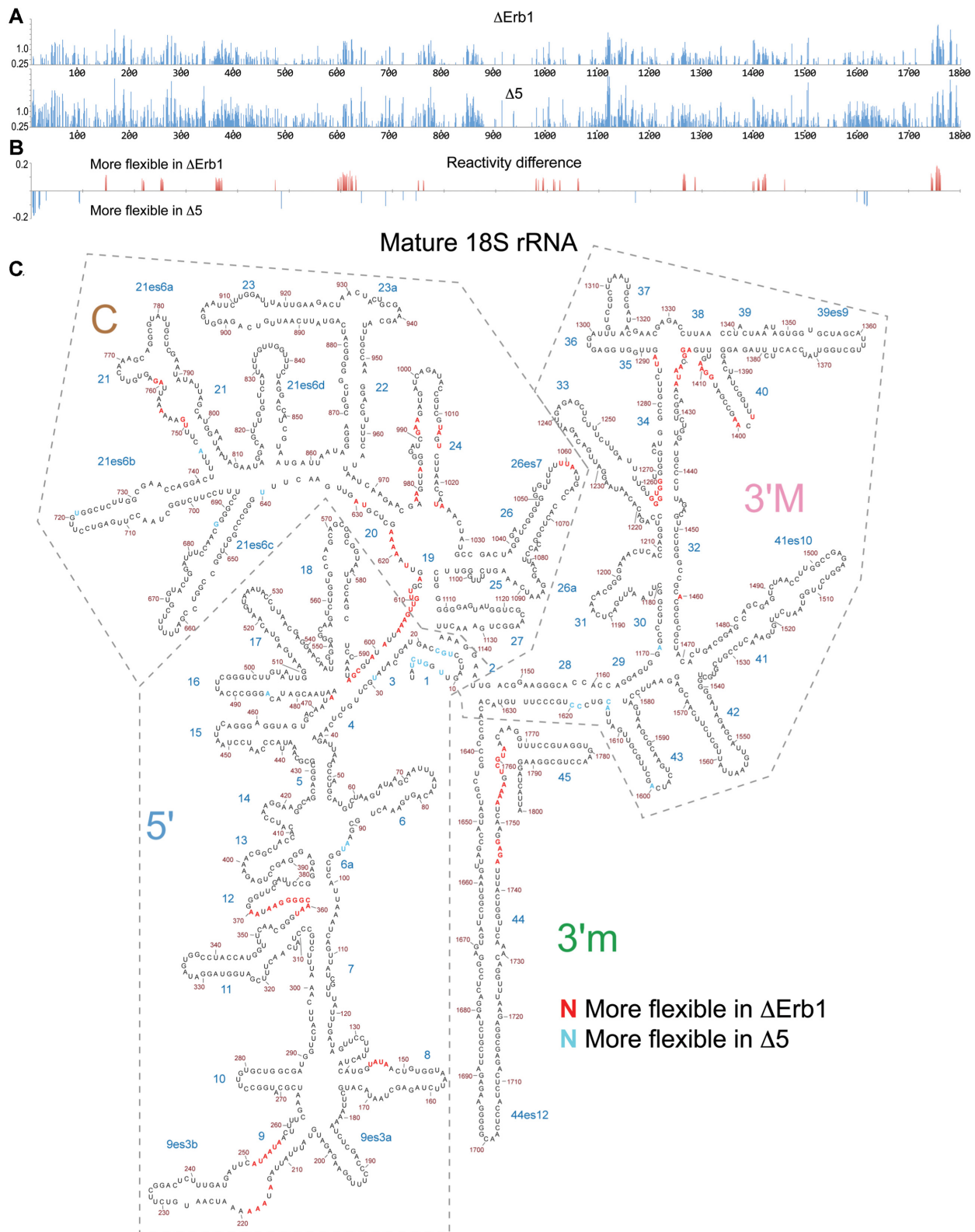
Figure 4. SHAPE reactivity pattern for the 18S rRNA region in 35S pre-rRNA. (A) ChemModSeq analysis of SHAPE reactivities of the 18S rRNA region in 35S pre-rRNA in \Delta\text{Erb1} and \Delta 5 . (B) \Delta\text{SHAPE} differences between \Delta\text{Erb1} and \Delta 5 that overlap with the BUM-HMM probabilities \geq 0.95 . Data analysis as in Figure 3. Red bars represent nucleotides with more reactivity in \Delta\text{Erb1} and blue bars nucleotides more reactive in \Delta 5 . (C) Distribution of SHAPE reactivity differences between \Delta\text{Erb1} and \Delta 5 in 18S rRNA within 35S pre-rRNA. Reactivity differences from Figure 4B are marked in the mature 18S rRNA secondary structure. Red marks nucleotides where \Delta\text{Erb1} reactivity is higher and blue marks nucleotides where \Delta 5 is higher. Domains in the 18S rRNA are indicated by dashed lines.
