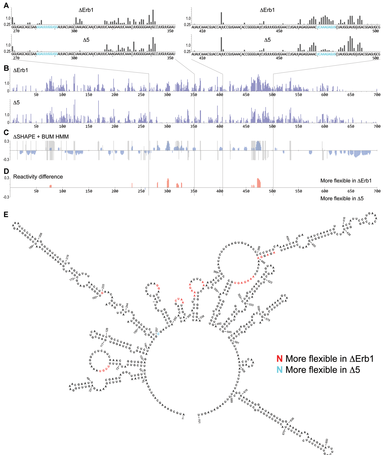
Figure 3. SHAPE reactivity pattern for the 5'ETS region in 35S pre-rRNA. (A) Primer extension determined SHAPE reactivities of nucleotides 268–350 (left) and nucleotides 405–504 (right) in \Delta Erb1 and \Delta 5. U3 base pairing sites, proposed in (20–23), are shown in blue. (B) ChemModSeq analyses for the entire 5'ETS (nucleotides 1–700) of 35S pre-rRNA in \Delta Erb1 and \Delta 5. (C) Comparison of SHAPE reactivities in \Delta Erb1 and \Delta 5, using \Delta SHAPE analyses and BUM-HMM probabilities. Blue bars show the \Delta SHAPE values. Gray regions mark nucleotides with posterior probabilities of \geq 0.95 according to BUM-HMM analyses for \Delta Erb1 (top) and \Delta 5 (bottom). (D) \Delta SHAPE reactivity differences between \Delta Erb1 and \Delta 5 that overlap with the BUM-HMM probabilities. In red, more flexibility in \Delta Erb1, in blue, more flexibility in \Delta 5. The regions analysed by primer extension are indicated by dashed lines. (E) Reactivity differences marked in a secondary structure model of the 5'ETS (44). Red nucleotides were more reactive in \Delta Erb1, blue nucleotides were more reactive in \Delta 5.
