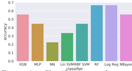
Figure 3: Classification performance over each script.
