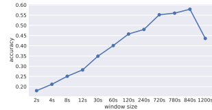
Figure 2: LR performance over various window sizes.
